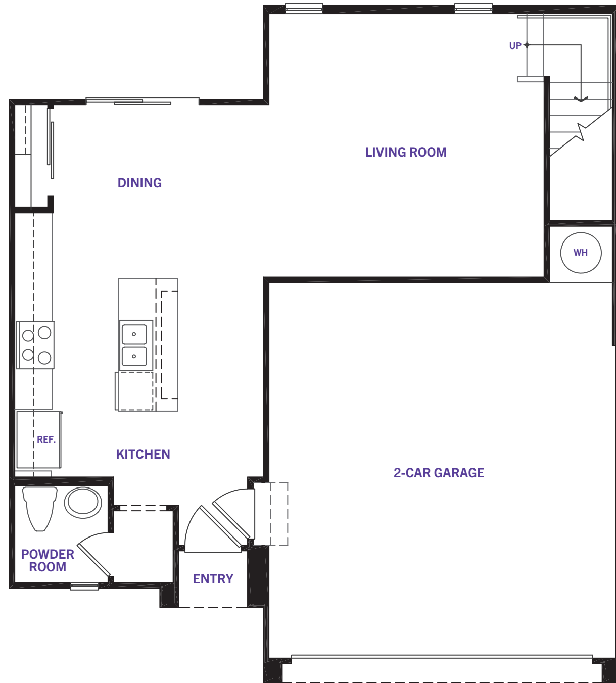
FIRST FLOOR
