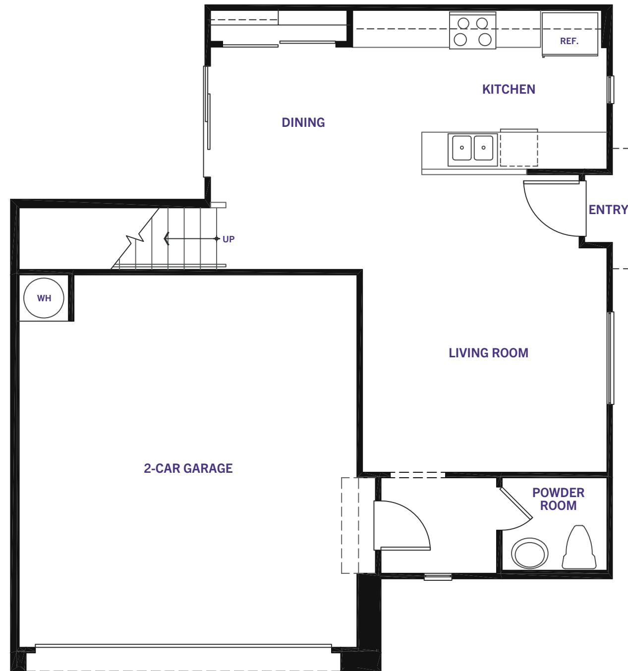
FIRST FLOOR
