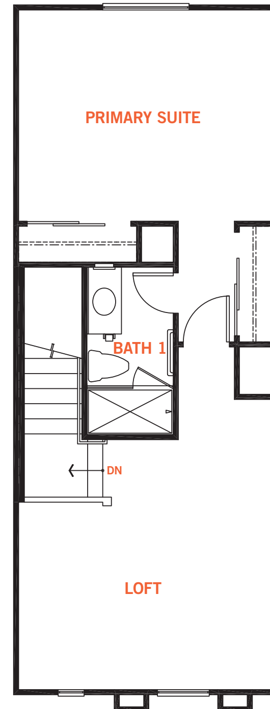
THIRD FLOOR
