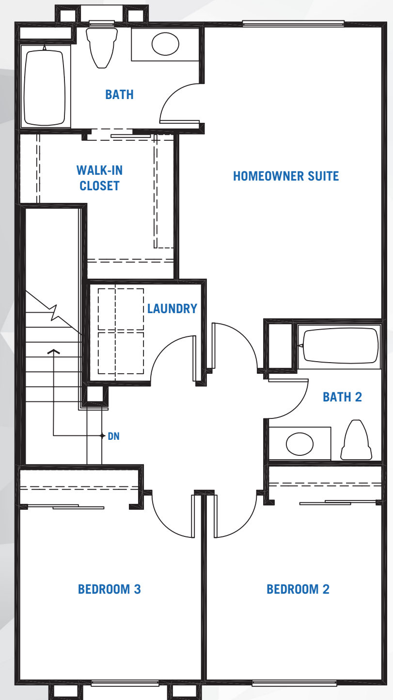
THIRD FLOOR
