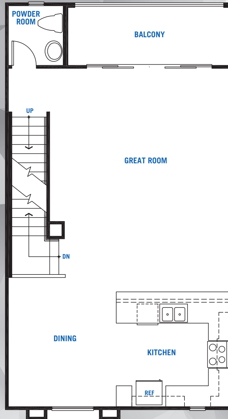
SECOND FLOOR
