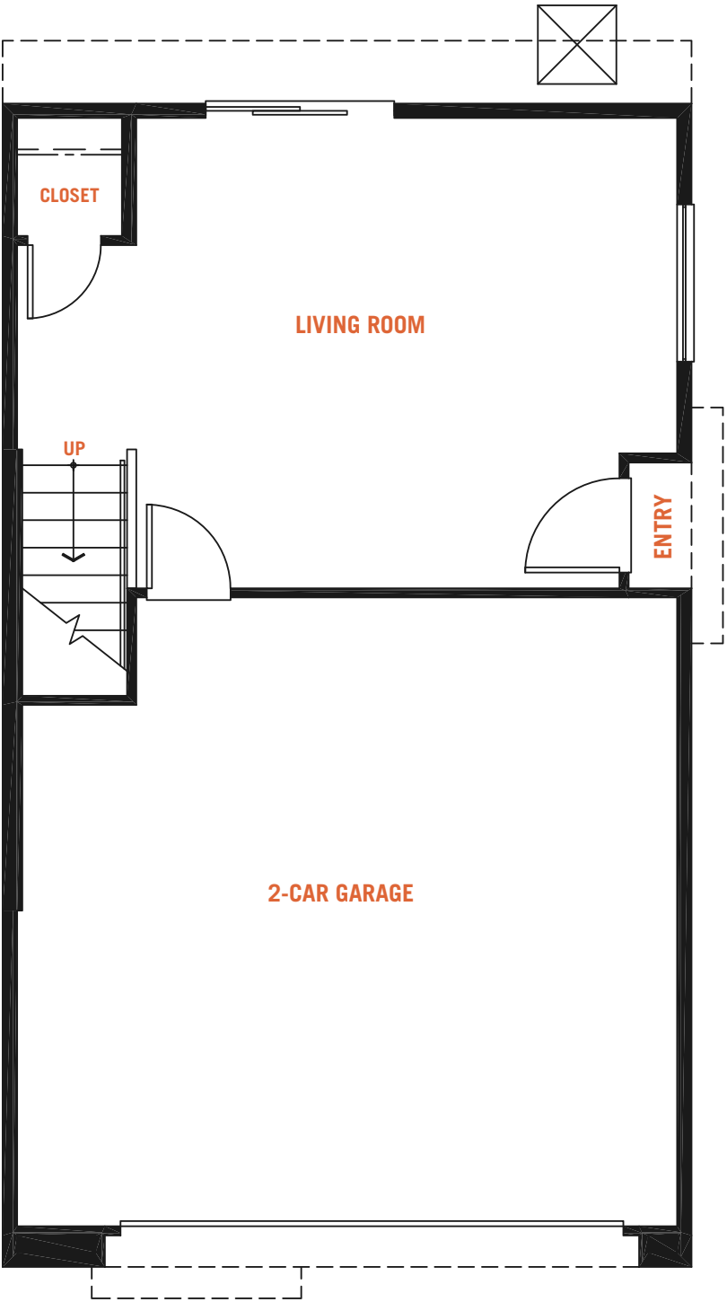
FIRST FLOOR
